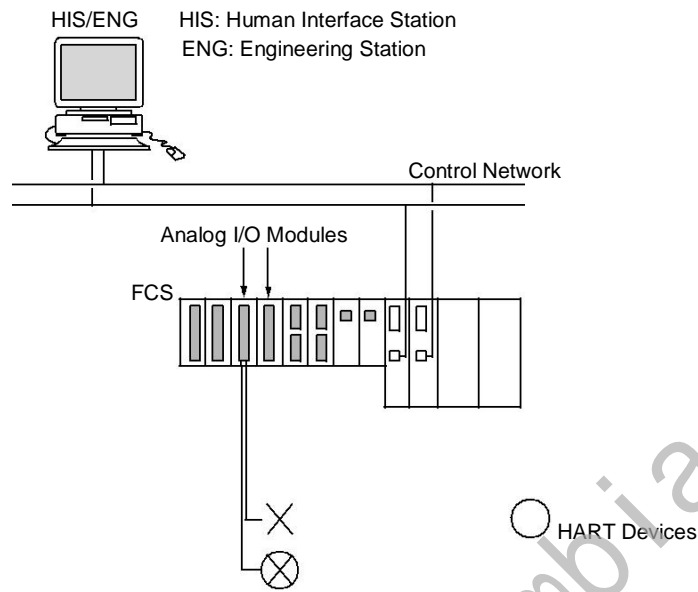
Figure HART Communication System Configuration (Dual-redundant)
